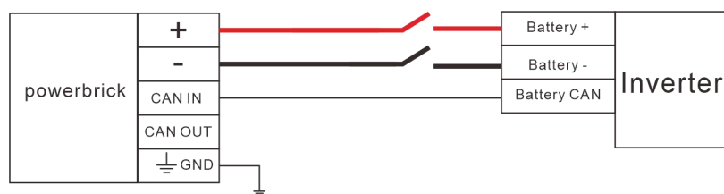
Figure 3-5 Wiring diagram
